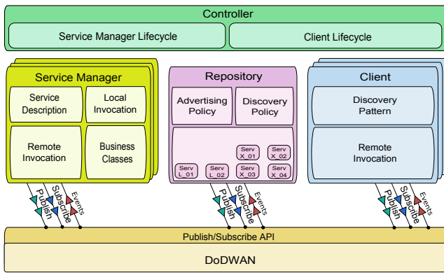
Figure 2. Architecture of the service platform
