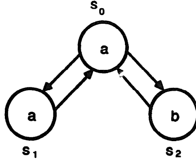
Fig. 1. A Kripke structure in which every other state is labelled A.
