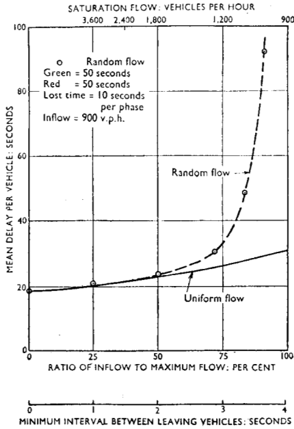
MEAN DELAY AT A FIXED-TIME TRAFFIC SIGNAL. RANDOM AND UNIFORM FLOW
