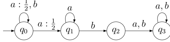
Figure 2.2: The MDP described in Example 2.3 with the initial Dirac distribution q_0 .
