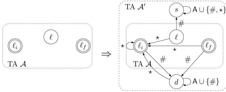
Figure 7.4: The reduction sketch to show undecidability of the (location-)synchronizing problem in TAs where in this example: \{l_i, l_f\} \subseteq F .
