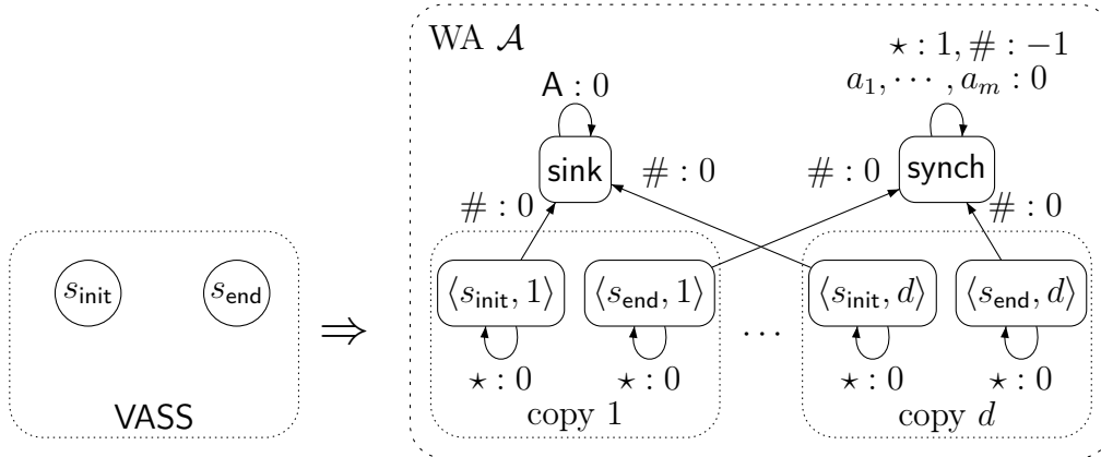
Figure 8.2: (Schematic) reduction from the coverability problem in vector addition systems with states to location-synchronizing problem from a subset S of locations under lower-bounded safety conditions in WAs.
