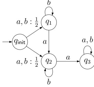
Figure 3.9: An MDP such that q_{\text{init}} \in \langle\langle 1 \rangle\rangle_{\text{sure}}^{\text{event}}(q_2) implying that the MDP is sure eventually synchronizing in \{q_2\} by some strategy. However, there is no blind strategy under which the MDP is sure eventually synchronizing in \{q_2\} , and thus \mathcal{L}_{\text{sure}}^{\text{event}}(q_2) = \emptyset from q_{\text{init}} when interpreting the model as a PA.
