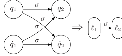
Fig. 2. Transitions between twin states q_1, \hat{q}_1 and q_2, \hat{q}_2 .
