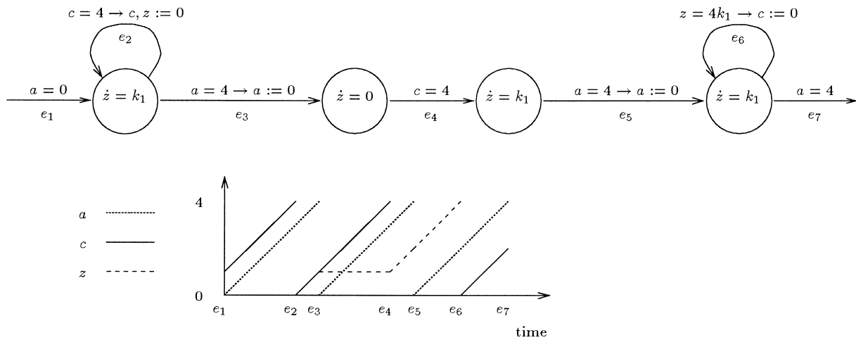
FIG. 20. Doubling c using the two-slope variable z with the slopes 0 and k_1 .
