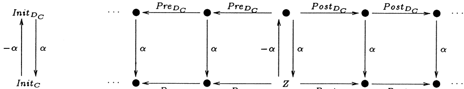
FIG. 3. Commuting diagram for zones Z of an initialized stopwatch automaton C .
