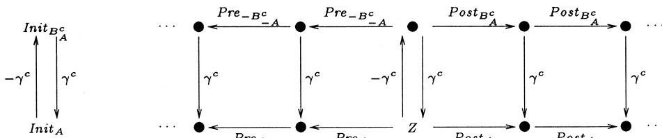
FIG. 8. Commuting diagram for compact rectangular zones Z of a compact initialized rectangular automaton A .
