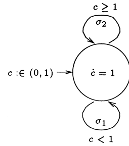
FIG. 10. The initialized rectangular automaton \bar{A} for which Lang^c(\bar{A}) is not limit-closed.
