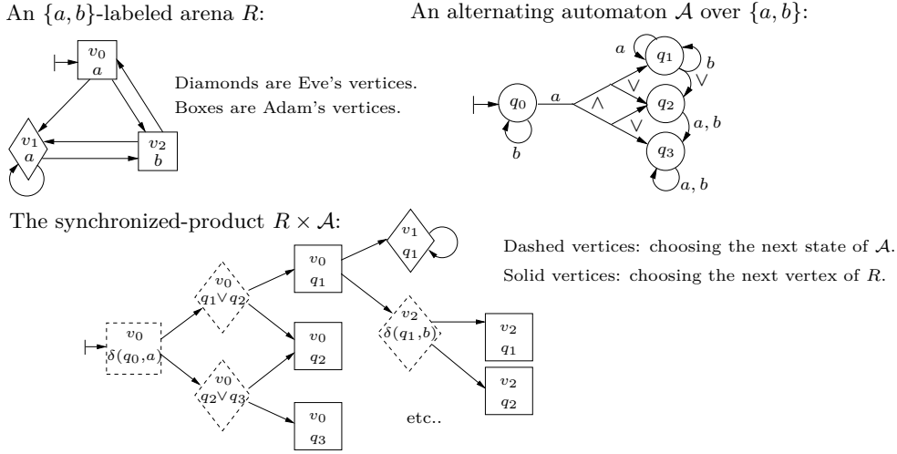
■ Figure 1 An example of a product between an alternating automaton and a finite arena.
