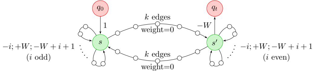
Figure 8: An example (with 2W + 2k + 2 states) showing that more than one cycle per state can be needed.
