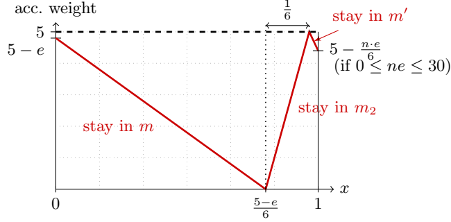
Fig. 6. The effect of module \text{Mod}_n
