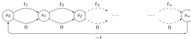
Fig. 3. Reduction from SUBSET-SUM
