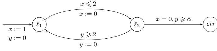
(a) A timed automaton \mathcal{A}_\alpha .
