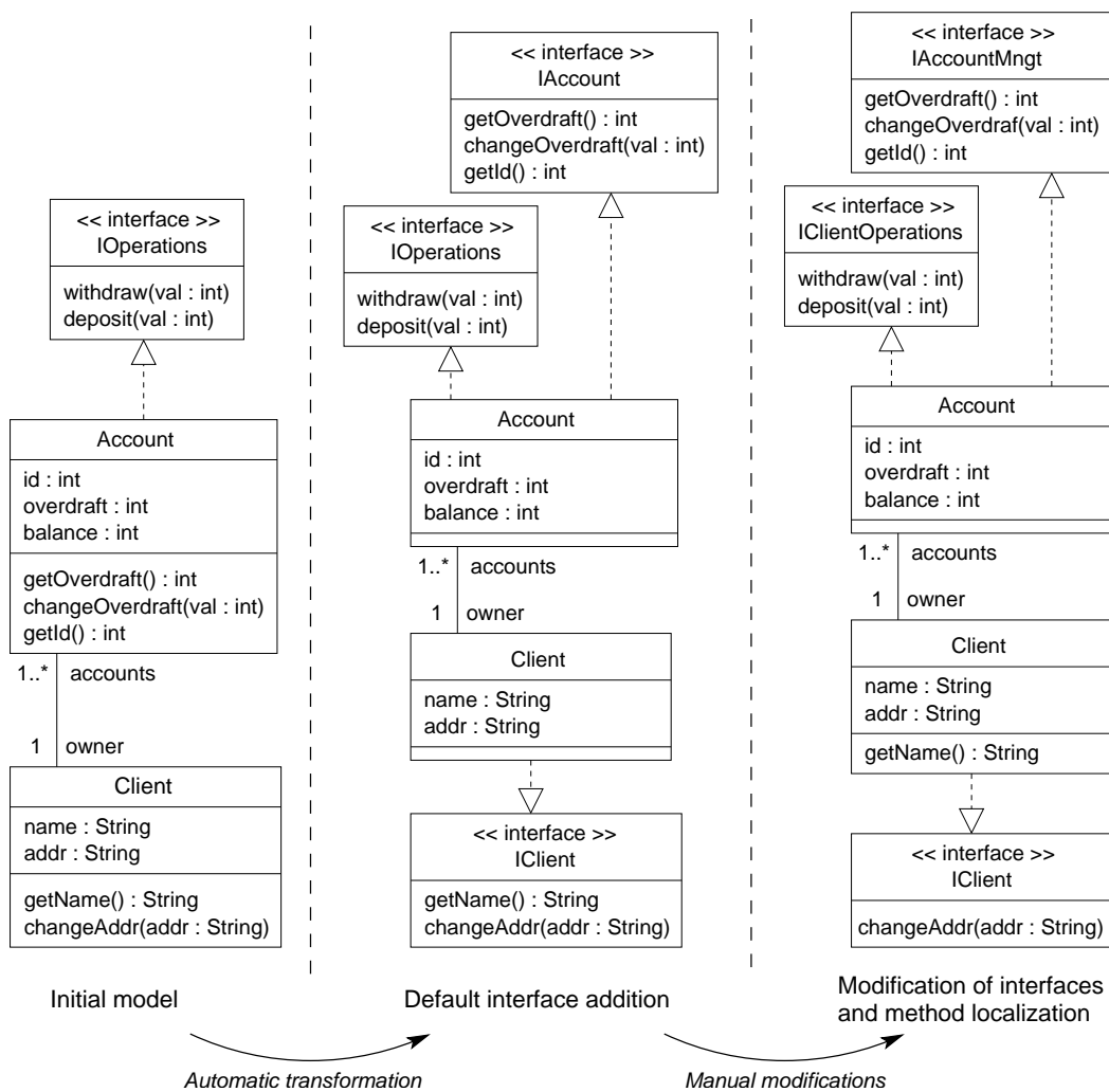
Figure 2: Refinement example: addition and modification of interfaces
