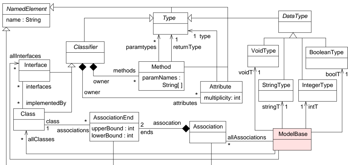
Figure 1: Meta-model of simplified class diagrams
