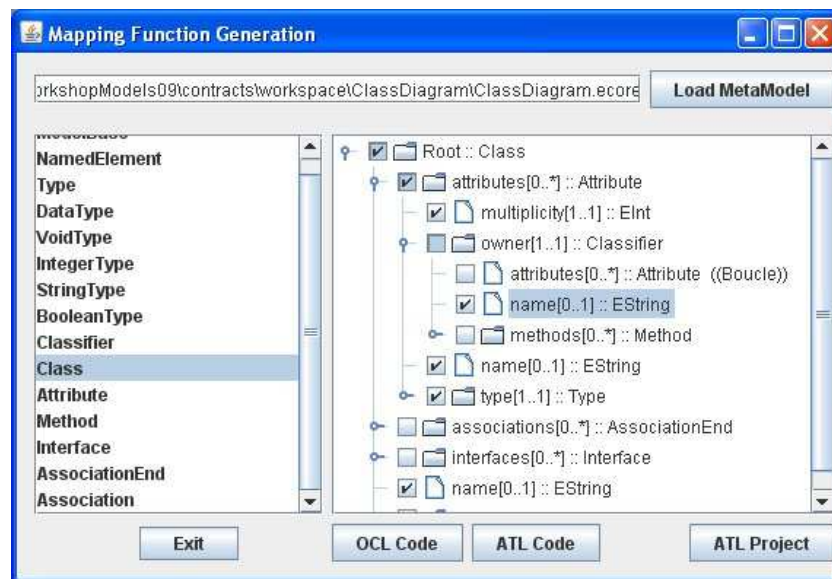
Figure 3: Mapping function generation tool: selection for class mapping
