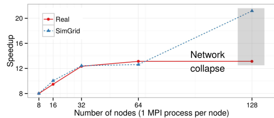
Figure 10: Evolution of the simulated and actual speedups for the CG benchmark on the graphene cluster.
