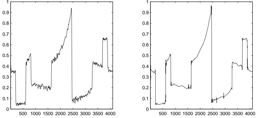
Figure 2.8: Estimation by using Wiener filter, with \lambda = \sigma^2 , SNR= 24.30 dB (left); estimation with a translation invariant soft thresholding, SNR= 31.50 dB (right)
