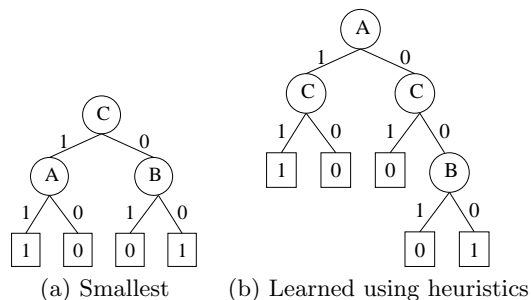
Figure 5: Two accurate trees for database 2
