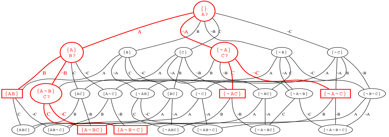
Figure 2: An itemset lattice for items \{A, -A, B, -B, C, -C\} ; binary decision tree A(B(C(1,1),1),C(1,1)) is hidden in this lattice
