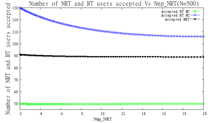
Fig. 10. Number of NRT and RT users accepted Vs Nnp\_NRT
