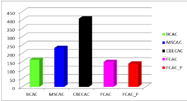
Fig. 14. Number of NRT users accepted for different CACs
