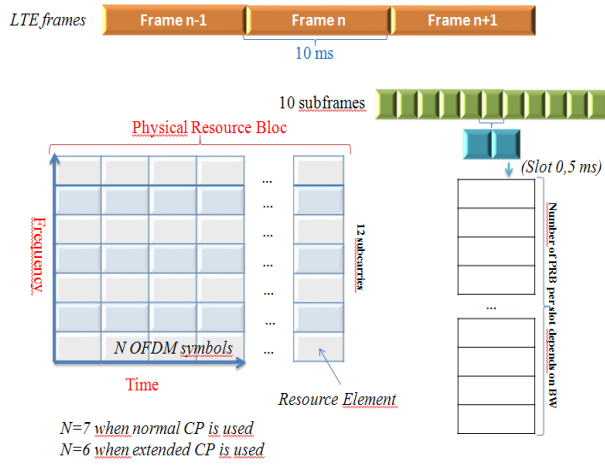
Fig. 7. Radio resources structure
