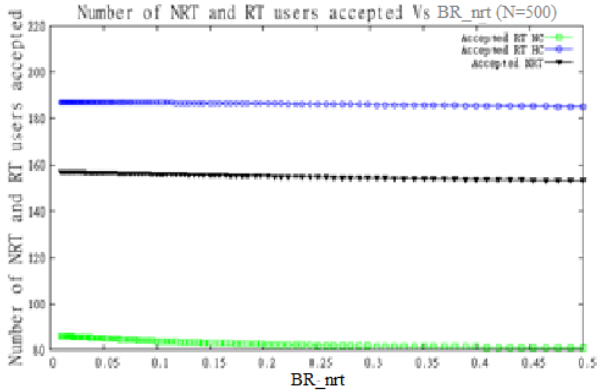
Fig. 8. Number of NRT and RT users accepted Vs BR\_nrt
