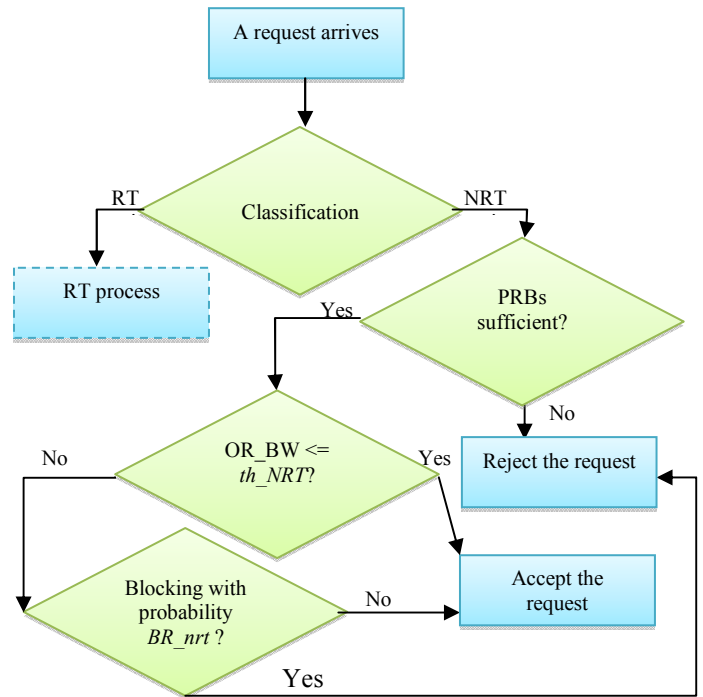
Fig. 4. General scheme in FCAC
