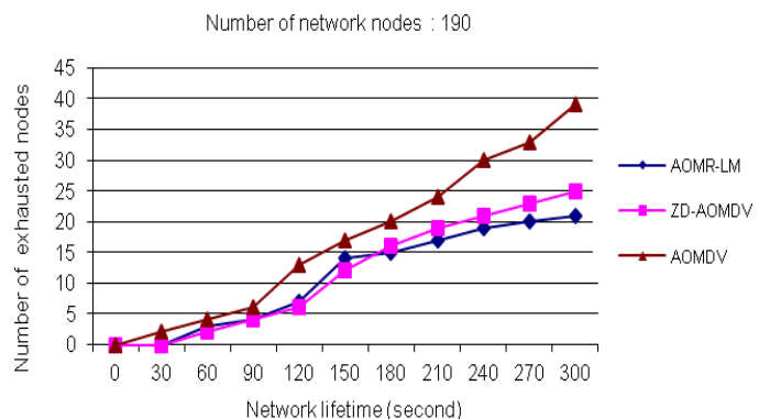
Figure 3: Network lifetime versus number of exhausted nodes.
