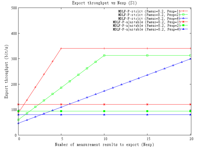
Fig. 2. Average export throughput vs N_{exp} when FDLM-P-strict and FDLM-P-adjustable are used.
