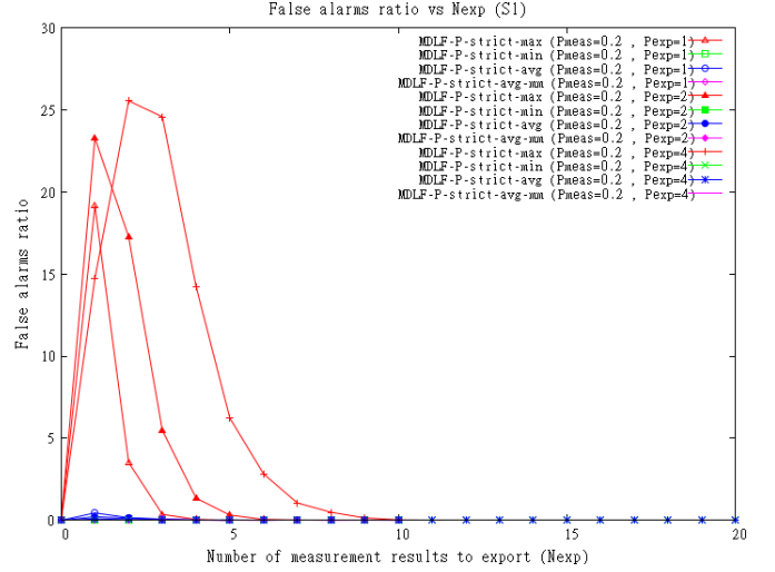
Fig. 4. False alarms ratio vs N_{exp} when FDLM-P-strict is used.
