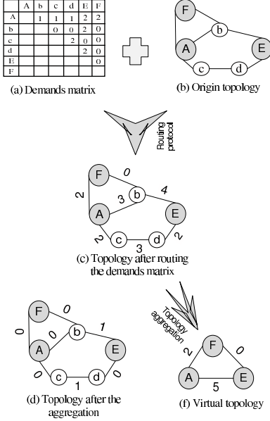
Figure 6. Topology aggregation model
