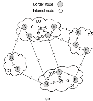
Figure 3. Multi-domain optical networks
