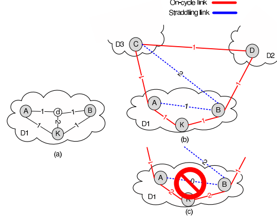
Figure 7. Proposed model of topology aggregation
