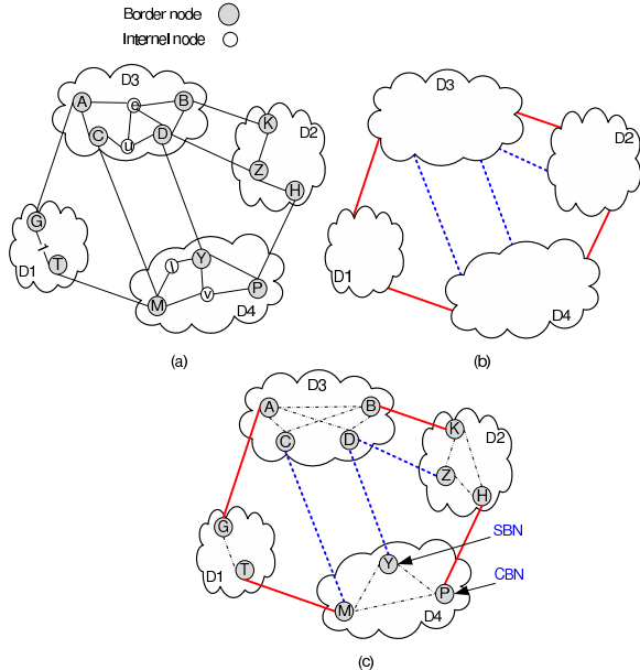
Figure 2. Multi-domain protection using p-cycle
