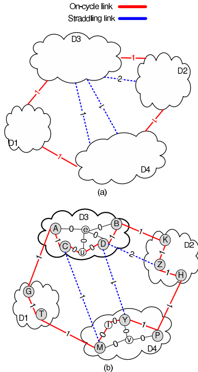
Figure 5. Computed p-cycles with single-virtual-node domains
