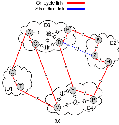
Figure 4. Computed p-cycles with internal topological knowledge
