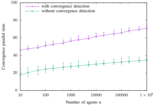
Figure 8. Comparison of the parallel convergence time of proportion computation with convergence detection and without convergence detection as a function of n , with N = 10^3 and \varepsilon = 10^{-5} .
