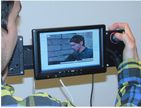
Figure 4: Our hand-held virtual camera device with custom-built dual handgrip rig and button controls, a 7-inch LCD touch-screen.
