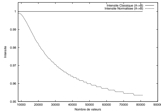
FIG. 6 – cas où n(a) = 1296 , n(b) = 2304 , n(a \wedge b) = 1296 , s_0 = 0 , c_0 = 0
