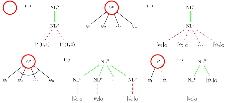
Fig. 4. Transformation of an ADTerm into a game by means of function [\cdot]_{\mathbb{G}} .
