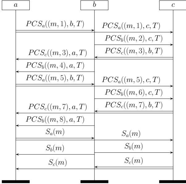
Figure 2. Protocol generated by Algorithm 1 from signing sequence (a, b, c, b, a, b, c)
