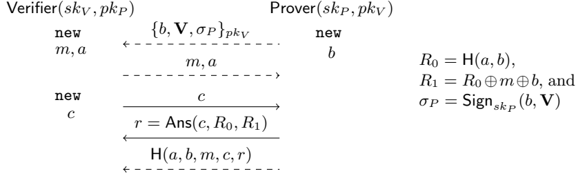
Fig. 1: Description of the SPADE ( fixed ) protocol
